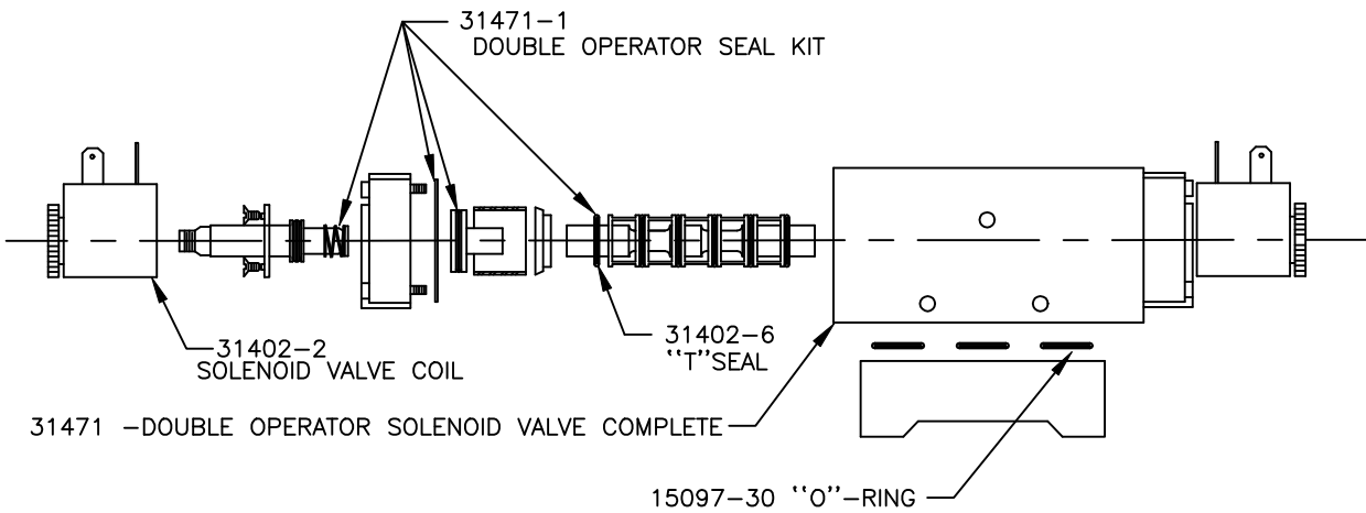
31471-DOUBLE OPERATOR SOLENOID VALVE
