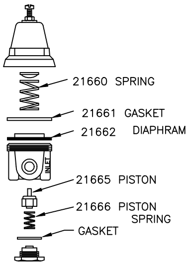
1/4"REGULATOR 16048
