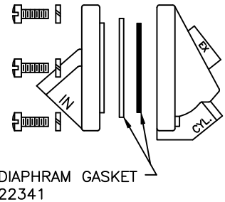
QUICK EXHAUST VALVE 17799
