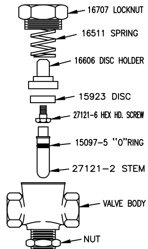
1/4" AIR WHISTLE VALVE 15100
